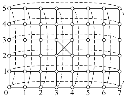
Fig. 2. Adding two edges in T_{8,6} to reduce the diameter by one.
